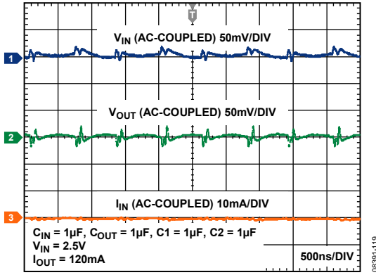
Figure 22. Typical Operating Waveforms, G = 2\times
