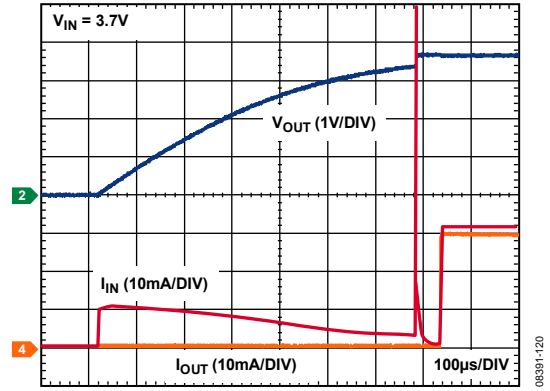
Figure 23. Typical Start-Up Waveform
